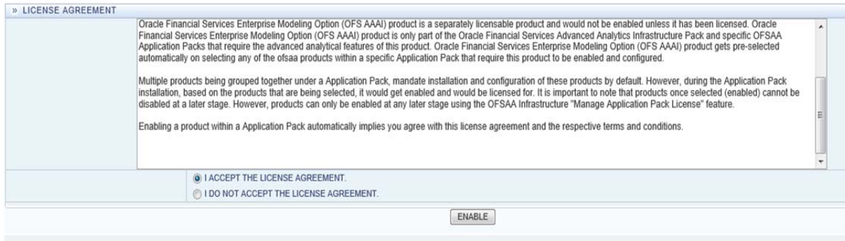
Figure 7–35 License Agreement
