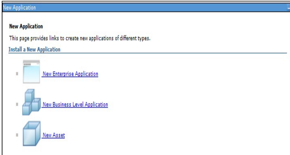
Figure 7-14 New Application
