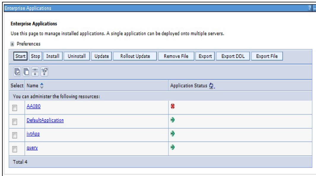
Figure 7-22 Enterprise Applications
