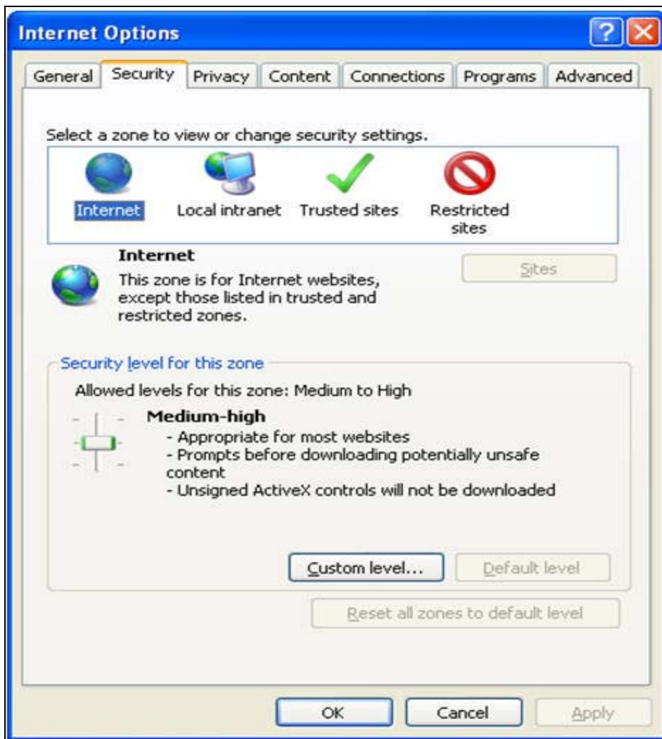
Figure 7-37 Internet Options
