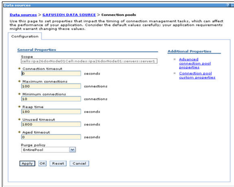
Figure 7–12 Connection pools
