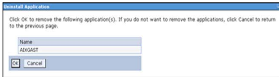
Figure 7–41 Uninstall Application
