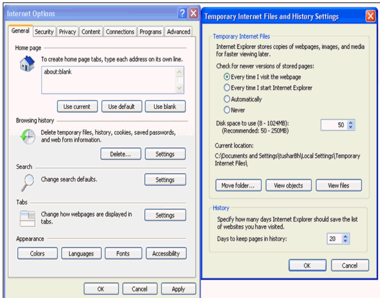
Figure 7–36 Internet Options
