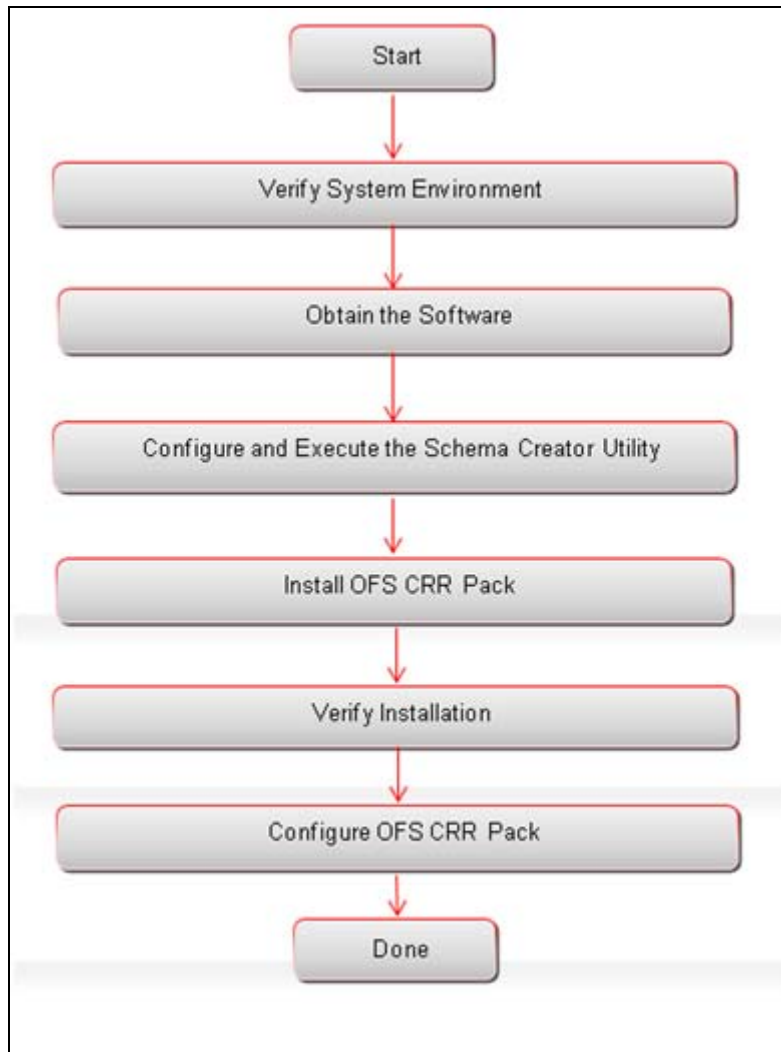
Figure 2–1 Installation Overview
